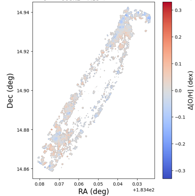
NGC4192: \Delta[\text{O}/\text{H}]_{\text{O3N2} - \text{M13}} (offset from bin mean)
