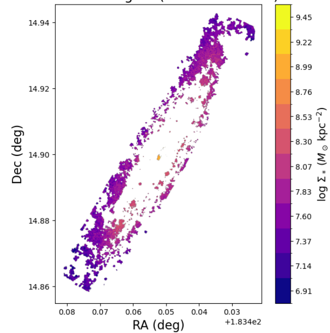
NGC4192: \log \Sigma_{*} (12 discrete bins)
