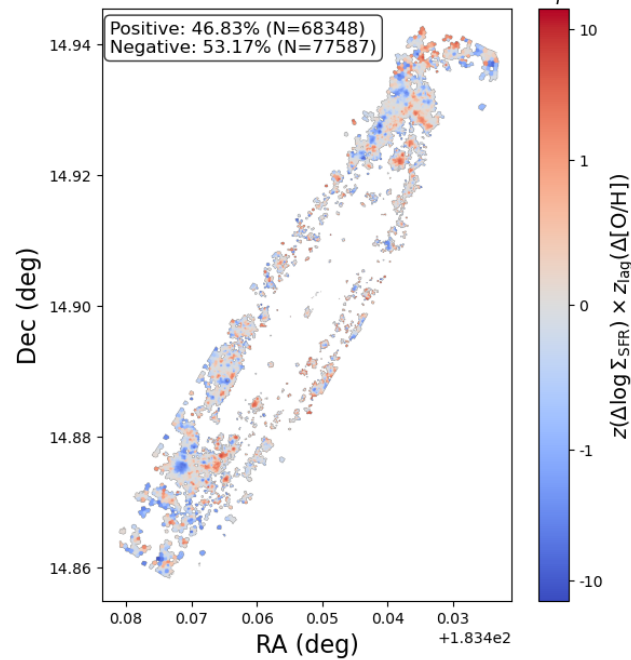
NGC4192: local bivariate Moran-like I_i
